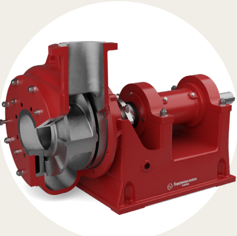
KBKM 150/300 dredger pump with free shaft end
